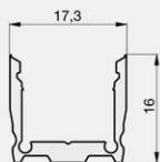
PROFILE SMALL U 17.3/16/B1C1 1M TRPA2501
