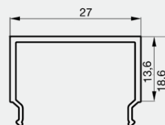
COVER MEDIUM SQUARE 27/14/C2 1M ZTPA3121
