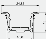
PROFILE SMALL WING 25/13/B1C1 1M TRPA2521
