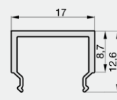
COVER SMALL SQUARE 17/9/C1 1M ZTPA3111
