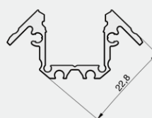
PROFILE SMALL CORNER 22.8/22.8/B1C1 1M TRPA2531
