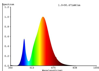
LED-Retrofit-Lampen 3000K
