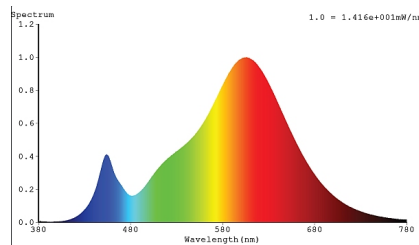
Lampes LED Retrofit 2700K
