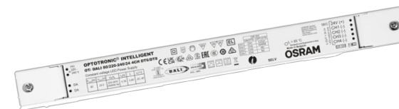
LED driver DALI, DRIVER DALI 4CH 80W/24V IP20
