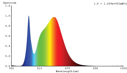
LED-Retrofit-Lampen 4000K
