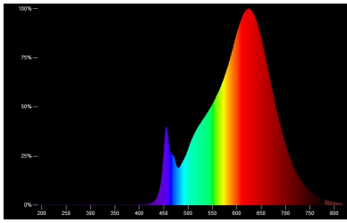
RaLEDina: LED retrofit for Linear incandescent lamp 2700K with best colour rendering CRI90
