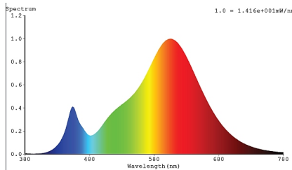
LED-Retrofit-Lamps 2700K
