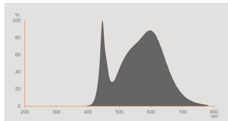
LED Retrofit reflector lamps 4000K
