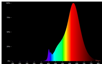
RaLEDina: LED retrofit for Linear incandescent lamp extra warm 2200K with best colour rendering CRI90
