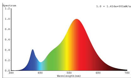
LED-Retrofit-Lamps 2700K
