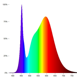
LED-NEO-Tubes 4000K, Replacements for fluorescent lamps
