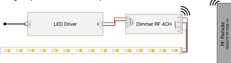
Wiring example for Tunable White LED Strips
