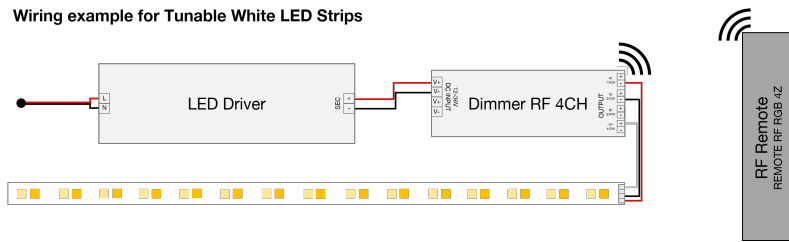
Wiring example for Tunable White LED Strips
