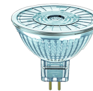
LED low voltage retrofit, RL MR16 35 4,6W/12/WFL/827/GU5.3
