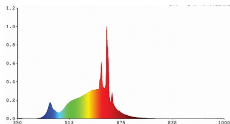
LED-Retrofit-Lamps 2700K
