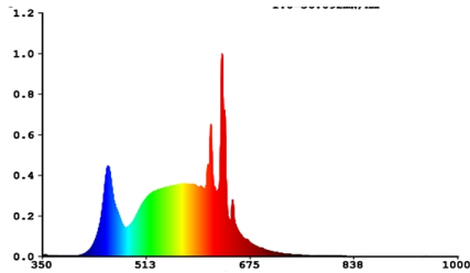
LED-Retrofit-Lamps 4000K, very good color rendering CRI 90
