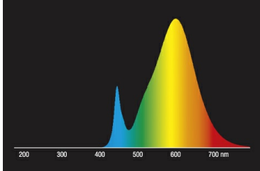
LED-Retrofit-Standardlampen 2700K
