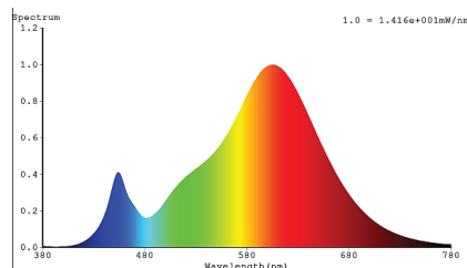
LED-Retrofit-Lampen 2700K
