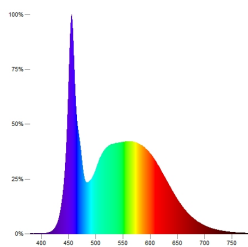
LED-NEO-Tubes 6500K, Replacements for fluorescent lamps
