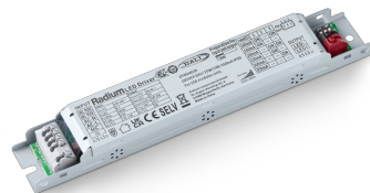
DALI-driver for DC-LED lamps and modules, DRIVER DC DALI 15W/100-350mA IP20
